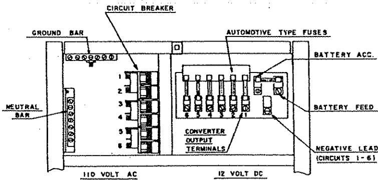
(FIG. 6) 45 AMP CONVERTER PANEL
