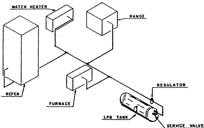
(FIG. 12) LP GAS SYSTEM (TYPICAL)
